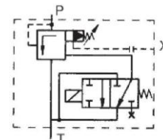
KPPE10/...TB-NO... 110/220 VAC 12/24 VDC
