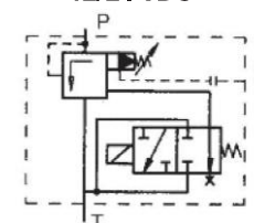
KPPE10/...TB-NZ... 110/220 VAC 12/24 VDC
